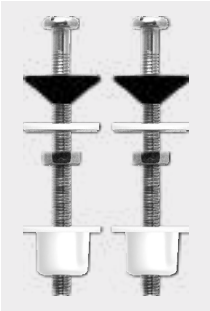
Tornillos TC 2 Ref. 0140564040 Packaging Bolsa 25 uds/caja PVP: 2,47 € Cisterna / WC RM 6 x 120 mm
