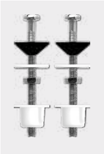
Tornillos TC 1 Ref. 0140564030 Packaging Bolsa 25 uds/caja PVP: 2,18 € Cisterna / WC RM 6 x 80 mm
